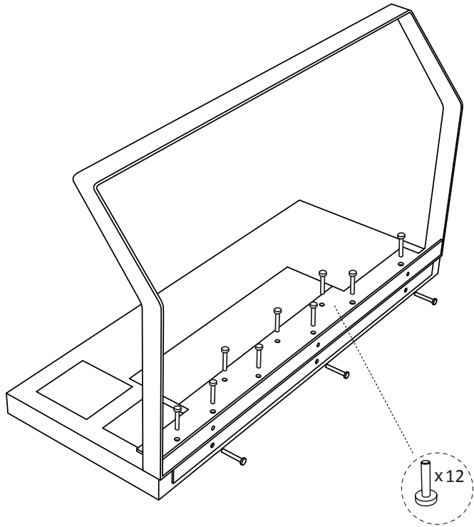
Mounting of frame to tabletop
